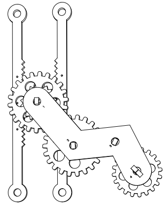
Bottom-Up view
